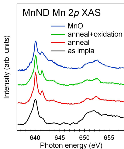
Fig.2 XAS spectrum of manganese-ion implanted nanodiamond with or without modification
