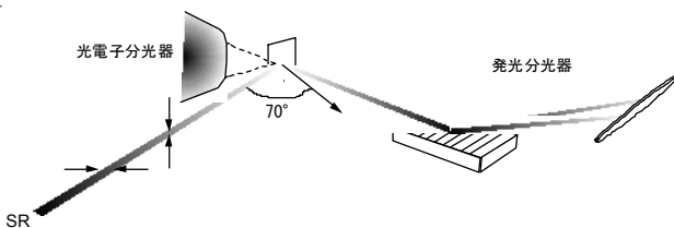
Fig.1 Schematic diagram of sample position
